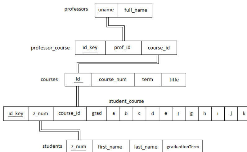
Figure 1.1 – Database model
